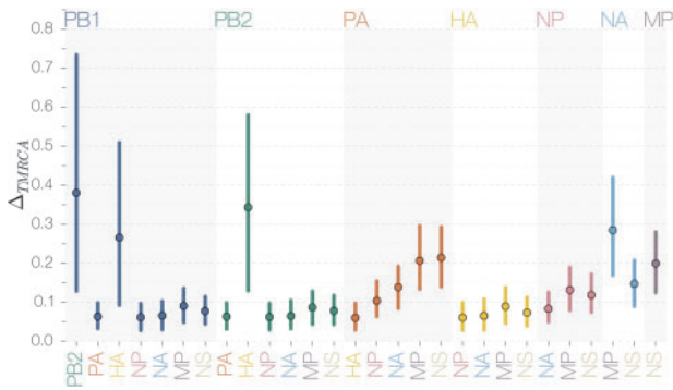
Fig. 8. \Delta_{\text{TMRCAs}} statistics for different segment pairs. PB1, PB2, and HA trees exhibit reciprocally highly similar TMRCAs, unlike most other pairwise comparisons. All vertical lines indicating uncertainty are 95% highest posterior densities.
